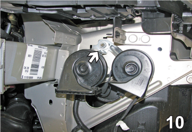
10. Using the 13MM socket, remove the metric bolt from the horn bracket on the driver side, unplug and set the bolt and horn aside to be reinstalled later.
