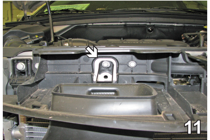
11. Using a 10MM socket, remove the metric bolt from the top of the air intake tube. Set the bolt aside to be reinstalled later.
