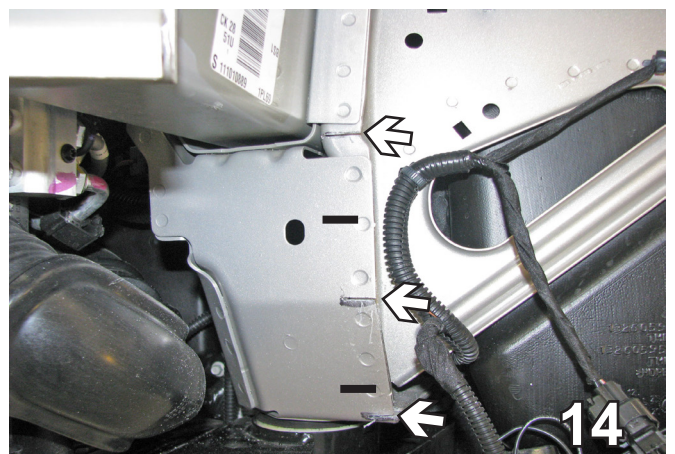
14. Cut frame webbing at the top, at the bend and at the bottom with a reciprocating saw. Be careful not to cut the main part of the frame. Do this on both sides.
