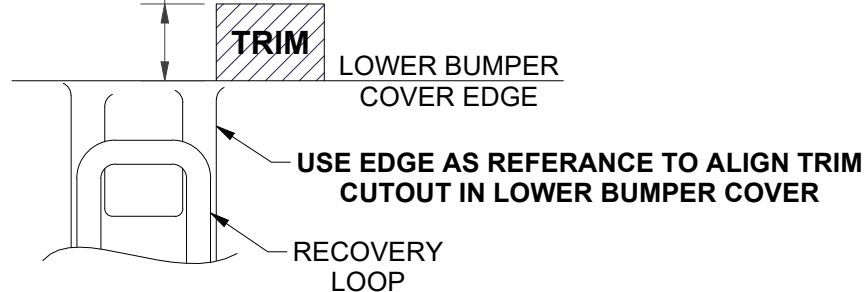
LOWER BUMPER COVER TRIM DIAGRAM
