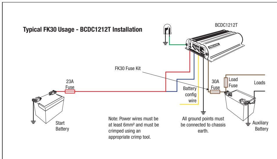
Diagram 2 - Typical FK30 Usage
