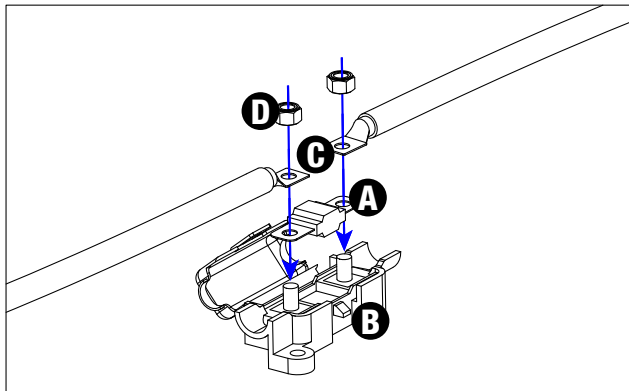
Diagram 1 - Fuse and Fuse Holder installation
