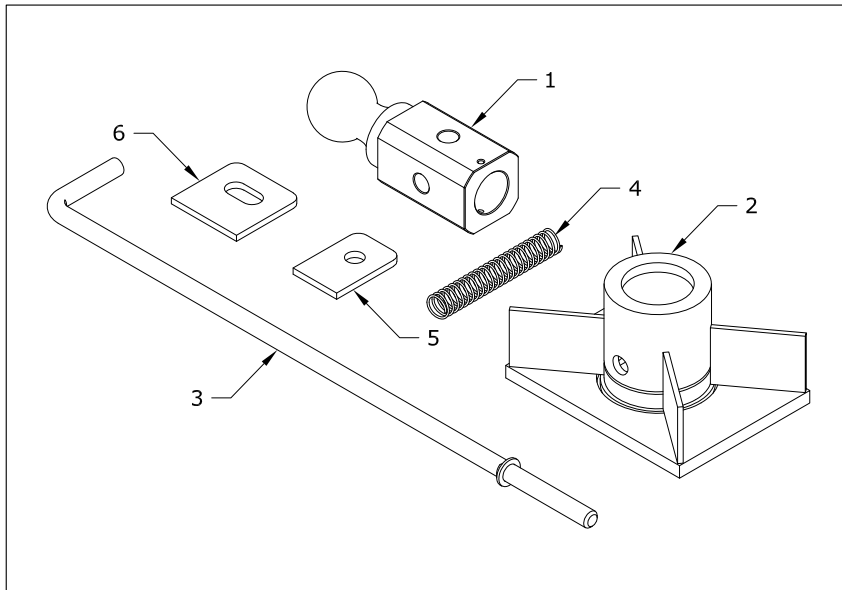
Kit Parts
