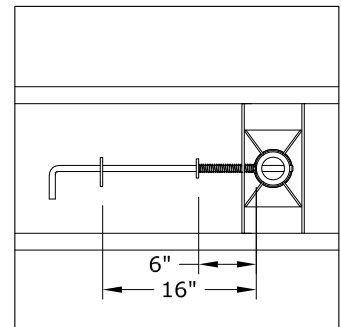
4.1 Install Latch.
