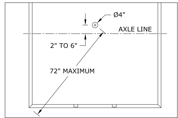
Top View of Truck Bed
