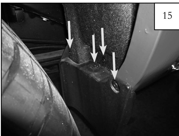
15 Using a T-15 Torx bit socket wrench, remove the four factory screws from the factory forward splash guard. Remove splash guard and discard.
