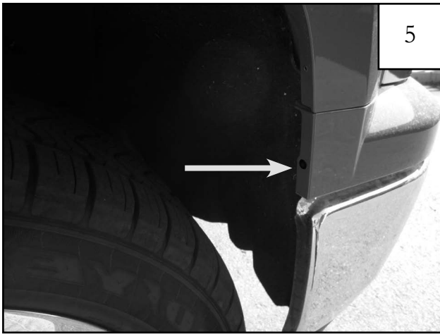
FOR 2014-2015 SILVERADO 1500 MODELS: Using a 7mm socket, remove factory screw at bottom front of wheel well.
