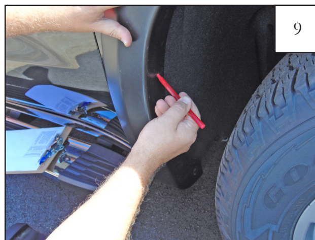
Use a grease pencil to mark the two locations of the holes indicated with the circles in Step 8. Remove flare from vehicle.
