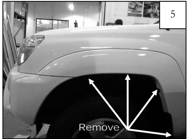
Remove four factory screws from the fender lip. Save screws for reinstallation. Remove flare by pulling part away from side of vehicle.
