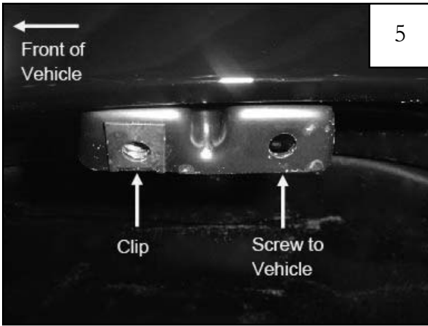
Install supplied plastic bracket using large Hex Screw into the plastic clip installed in step 10. The screw goes in rearward hole and the clip fastens over the forward hole.
