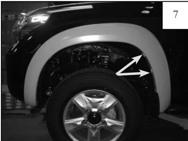
Install two supplied Plastic Tuf-Loks through rearward holes in Flare.
