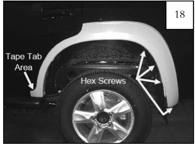
Reposition Rear Main Flare on fender. Hand start four supplied Hex Screws through flare and into hole locations shown (three in wheel well, one at rear underside of bumper). Do not tighten . Make sure that tape tab at front of flare is accessible.
