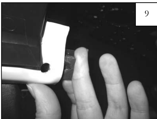
Slide "S" Clip/Black Tab combination onto sheet metal lip near rocker panel, at rear bottom of flare, aligning hole in clip with hole in flare.
