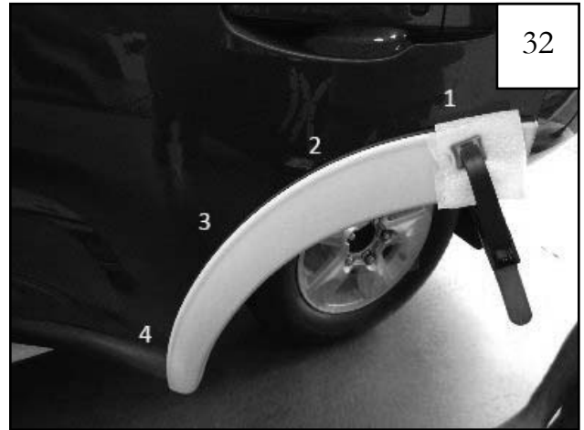
Using foam pad between the Door Piece and the ratcheting clamp, Attach clamp on upper part of Door Piece in position 1 and tighten. Leave clamp in place for 1 minute. Repeat clamping method for positions 2, 3 and 4. Leave clamp in place for 1 minute in each position.
