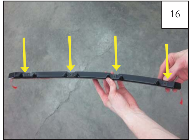
16 Inner Piece Clip (CL1-0023) locations (4 places). See next step (17) for a closer view of clip locations.
